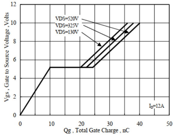
Fig 10 Gate-Charge Characteristics
