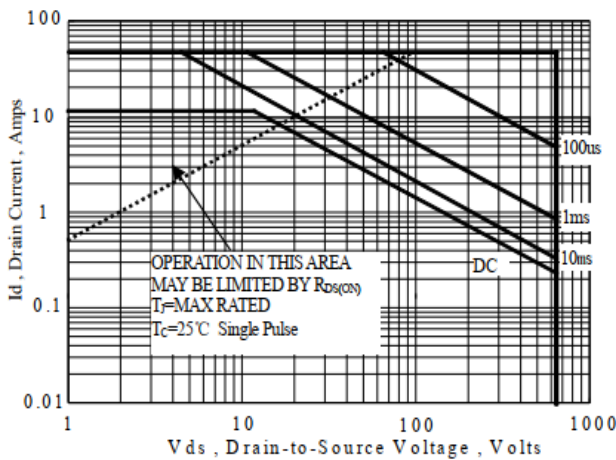
Fig 11 Safe Operating Area (TO-220AB / TO-263)
