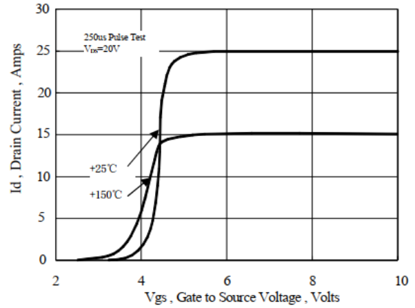
Fig 8 Transfer Characteristics
