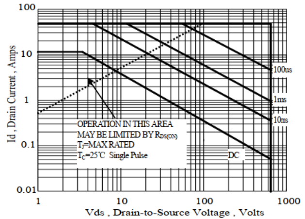
Fig 12 Safe Operating Area (ITO-220AB)
